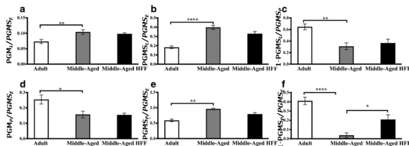
Figures 2 and 3. Respiratory flux control ratios and coupling control factors in hippocampus (2) and frontal cortex (3). Leak respiration with electron provision from complex I ( PGM_L / PGMS_E ) (a) and complexes I and II ( PGMS_L / PGMS_E ) (b), coupling efficiency of oxidative phosphorylation ( 1 - PGMS_L / PGMS_P ) (c), phosphorylating respiration with electron provision from complex I ( PGM_P / PGMS_E ) (d), and complexes I and II ( PGMS_P / PGMS_E ) (e), apparent excess capacity of the electron transport chain ( 1 - PGM_P / PGMS_E ) (f). Values are the means \pm SEM (N=8). * p < 0.05, ** p < 0.01, **** p < 0.0001
