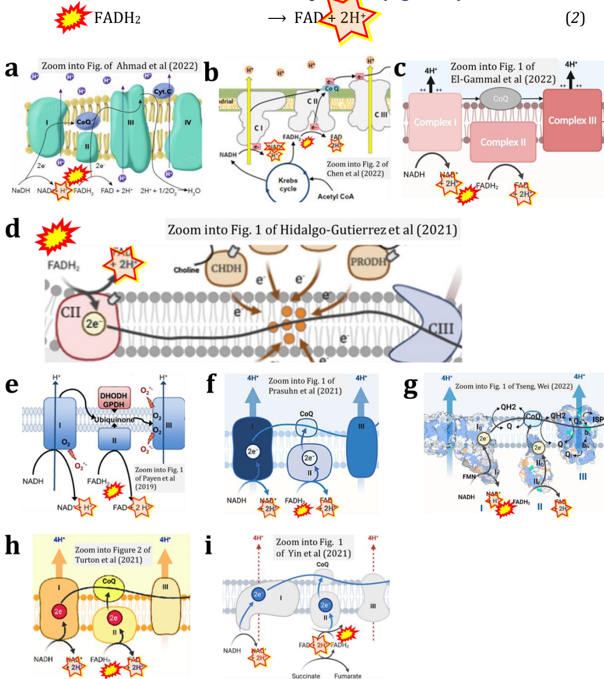
Figure S4. Complex II ambiguities: FADH 2 as substrate of CII and FAD + 2H + as products. Alphabetical sequence of publications from 2001 to 2023. See References for Figure S4.
