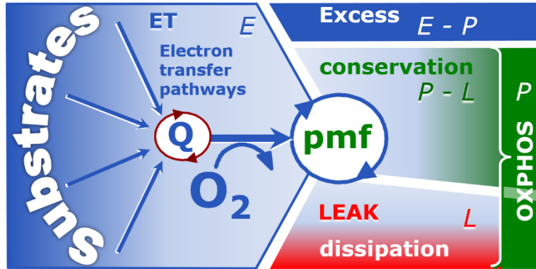
Figure 4. Four-compartment model of oxidative phosphorylation
